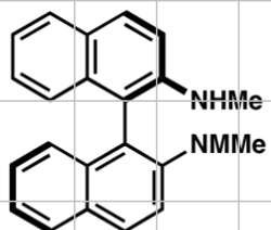
(R)-N,N-Dimethyl-1,1'-binaphthylidiamine
